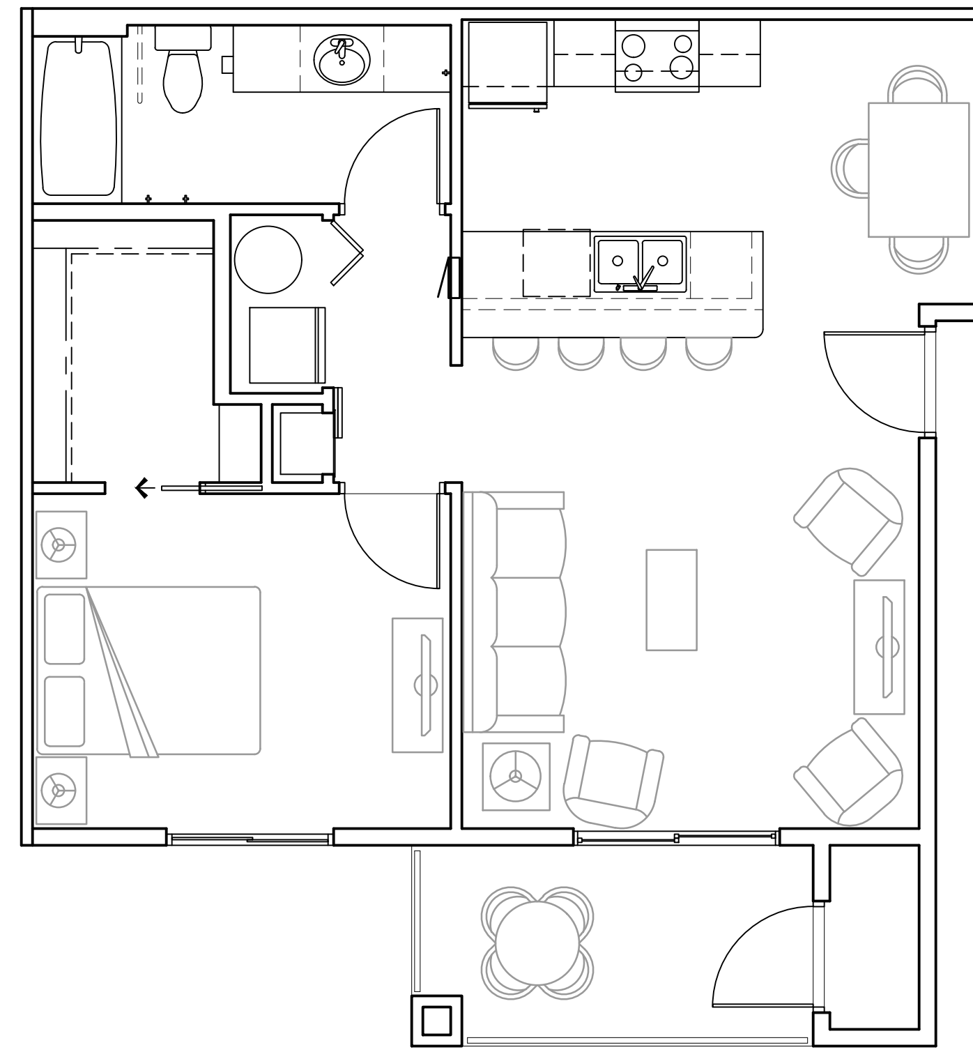
1 UNIT A FLOOR PLAN - 1-BED, 1-BATH SCALE: 1/4" = 1'-0"
